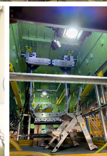
BRICK® lights used upper fuselage
