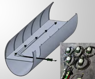
Medusa Configuration: (Up to 5 light heads, separate cords – individual light head control, 1 power box)
