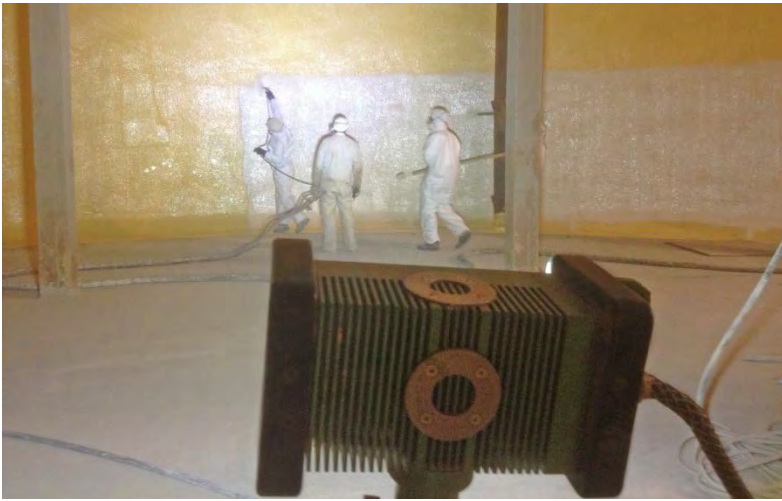
BRICK® mounted on self-propelled Blast & Paint unit for Penstock Pipeline
